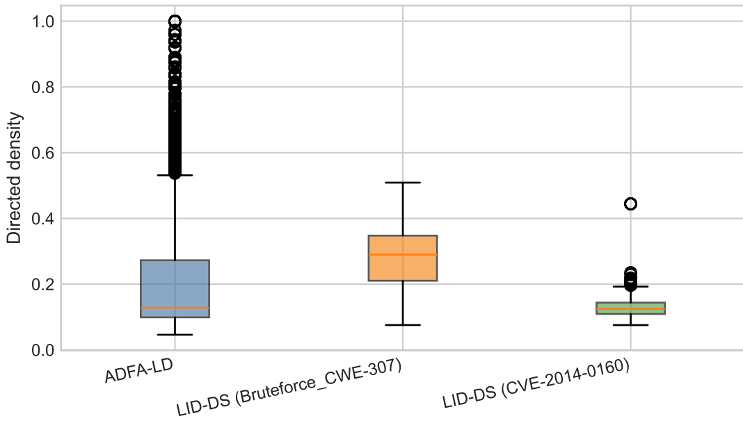
Graph density across datasets/scenarios
